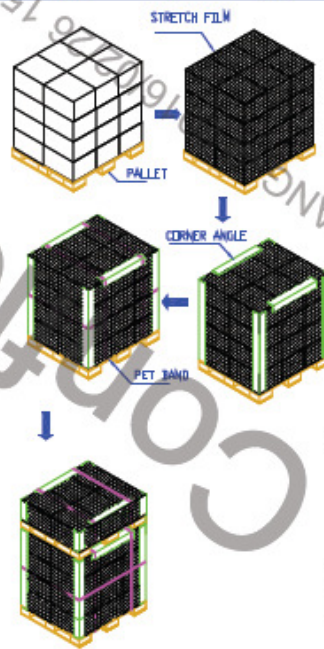
TWO PALLET SHIPMENT EXAMPLE SHIPPING BY SEA (USF) USED
